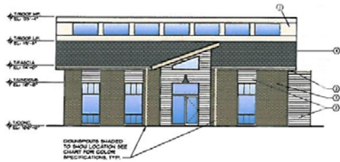
1 FRONT: OVERALL
