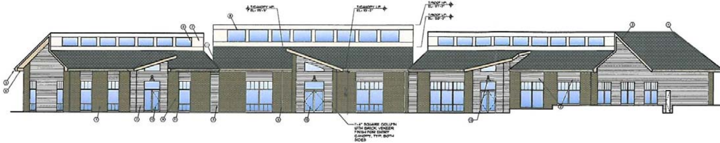
1 FRONT: OVERALL
